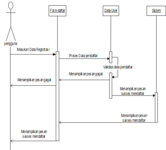
Gambar 6. Diagram Sequence
