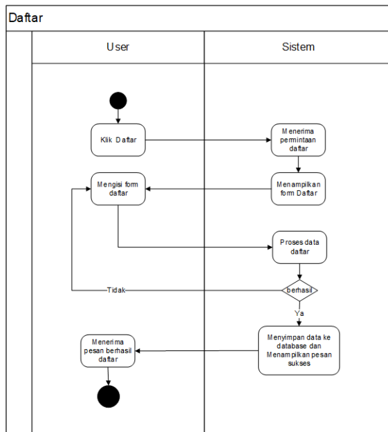
Gambar 5. Diagram Activity
