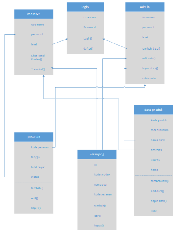
Gambar 7. Class Diagram
